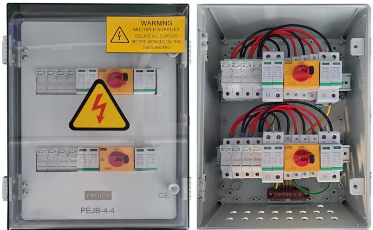
Photo 5 General Appearance of the EUT
